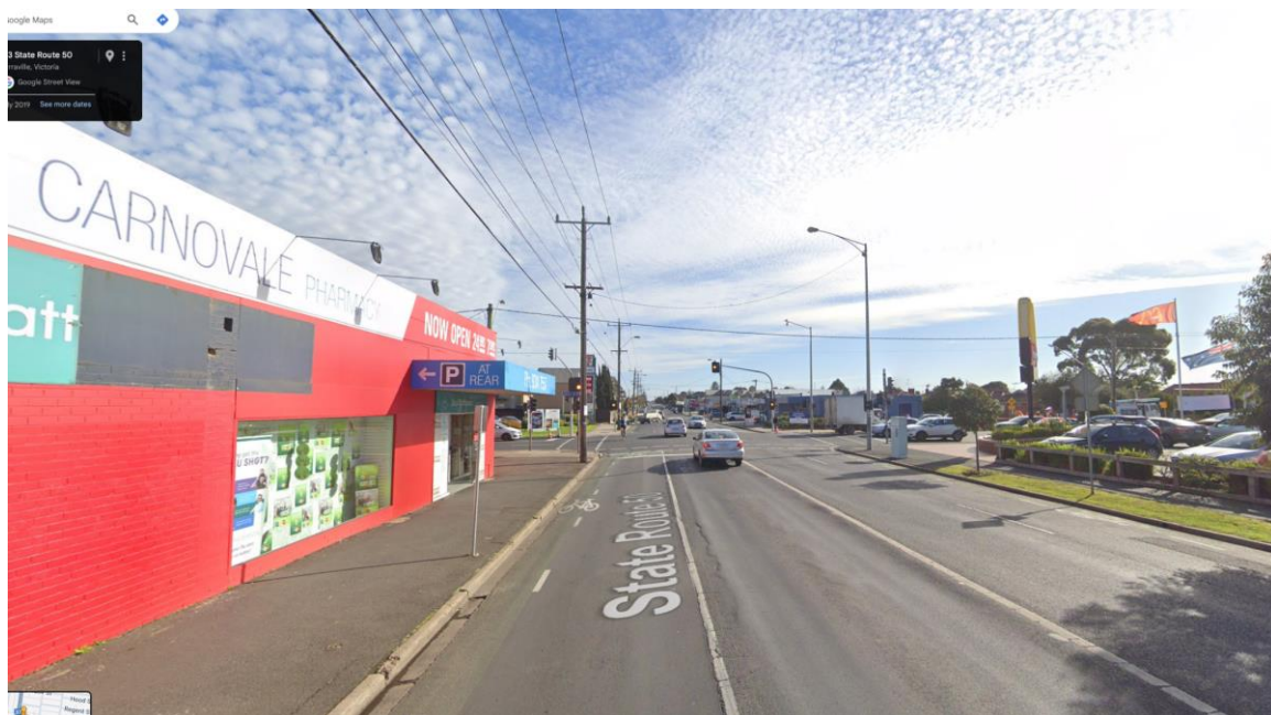
Figure 14: Too narrow bike lane (80cm) beside regular truck lane Yarraville (site of many recent collisions where cyclists were injured)
